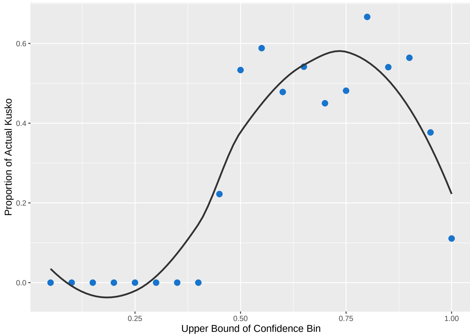
Proportion of Actual Kusko vs. Confidence Bins (Test Set)
